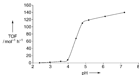
Figure 1. Initial TOF against initial solution pH values for the reduction of acetophenone (1 M, assuming the solution is homogeneous) by \text{HCOOH-NEt}_3 in water (1 mL total volume) with \text{Ru}-(R,R) -Ts-dpen at 40 °C. The initial pH values were determined by varying the \text{HCOOH/NEt}_3 molar ratios from 4.6:1.0 to 0.37:1.0.
