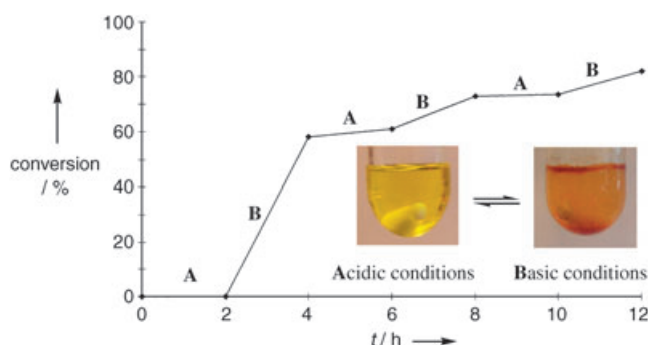
Figure 3. Graph of conversion versus time for the reduction of acetophenone (1 M) by HCOOH-NEt 3 in water (1:1 initial volume ratio, 0.5 mL water) with Ru-(R,R)-Ts-dpen at 40 °C. In regions A the initial HCOOH/NEt 3 molar ratio was maintained at 4.6:1.0 (pH 2.8), whereas in regions B HCOOH/NEt 3 = 2.3:1.0 (pH 3.7).
